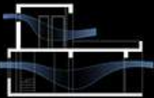
cross ventilation diagram
