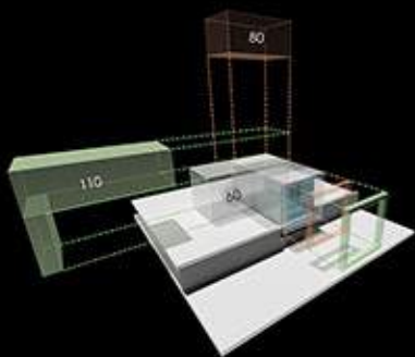
mechanism for generating the three size variations: 60m 2 , 80m 2 and 110m 2
